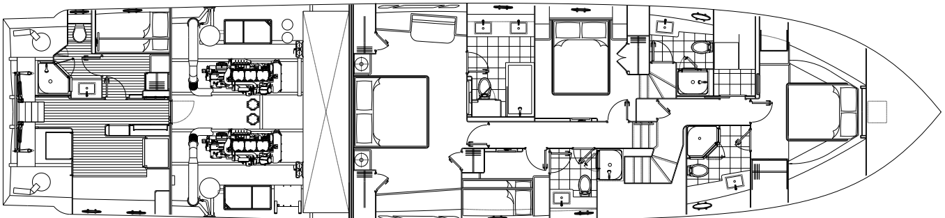
LOWER DECK PLAN
